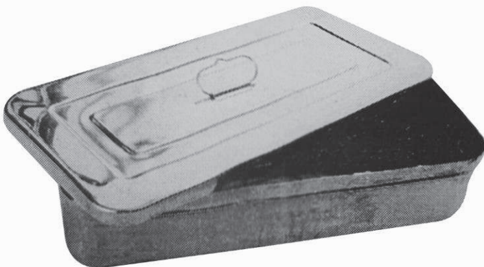
Code Size SB-1214-01 30 x 15 x 10 cm SB-1214-02 30 x 17 x 5 cm SB-1214-03 34 x 16 x 5 cm SB-1214-04 36 x 24 x 5 cm SB-1214-05 36 x 24 x 10 cm SB-1214-06 40 x 20 x 6 cm
